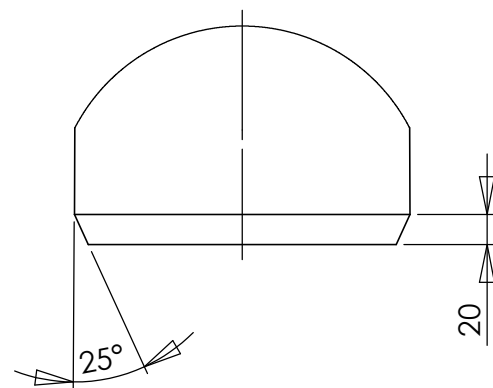
DETAIL C SCALE 1 : 5
