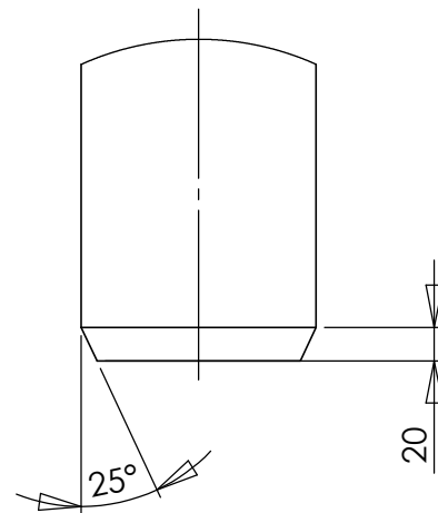
DETAIL C SCALE 1 : 5
